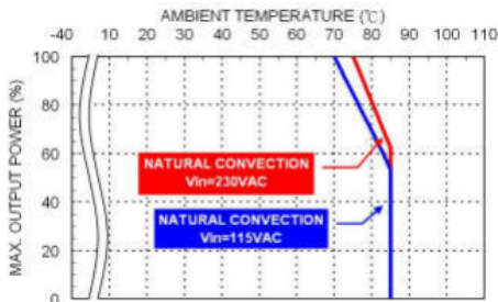
Derating Curve vs. Ambient Temperature 43MSD30USxxB xx=12/15/24/28/36/48/53 Connector Option : (0: JST)
