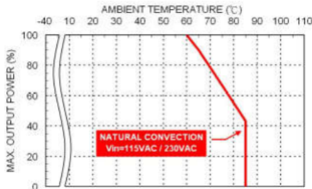
Derating Curve vs. Ambient Temperature 43MSD30USxxB xx=3P3/05/7P5/09/121/151/18 Connector Option : (0: JST)
