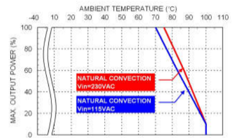
Derating Curve vs. Ambient Temperature 43MSD30USxxB xx=12/15/24/28/36/48/53 Connector Option : (-M / -T / -D)
