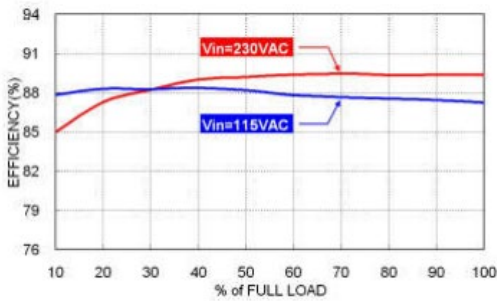
43MSD30US24B Efficiency vs. Output Load
