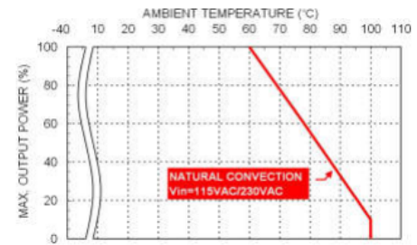
Derating Curve vs. Ambient Temperature MSD30USxxB xx=3P3/05/7P5/09/121/151/18 Connector Option : (-M / -T / -D)
